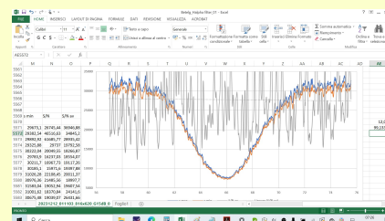
data analysis
