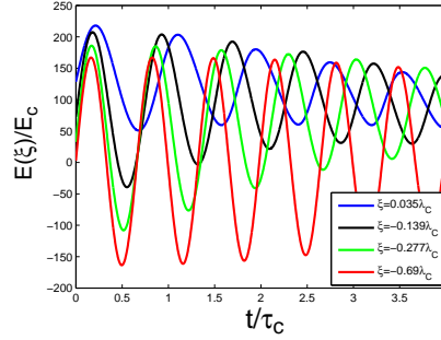
Figure C.2.: Time evolution of electric fields at different radial positions around the boundary layer of the baryon core, M = 10M_\odot , R_c \approx 10^7 \text{ cm} and v_p = 0.2c . The coordinate is \xi \equiv r - R_c .
