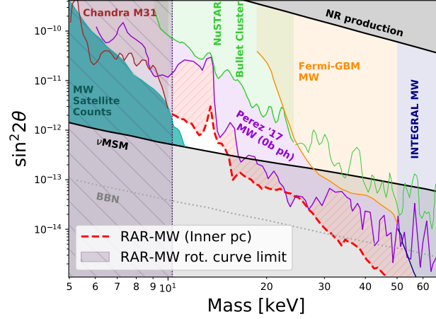
Figure 3.8: Sterile neutrino parameter space limits obtained for galactic center observations using RAR profiles, compared to previous bounds. Red-dotted line and 10.4 keV vertical shaded region correspond to RAR limits given by X-ray bounds and Milky Way rotation curve limits Argüelles et al. (2018a) respectively. Upper and lower grey shaded regions correspond to production mechanism bounds: NRP under no lepton asymmetry, \nu MSM for maximal model produced asymmetry and maximal BBN allowed values (see Yunis et al. (2018) for further details on other \nu MSM constraints corresponding to this figure).
