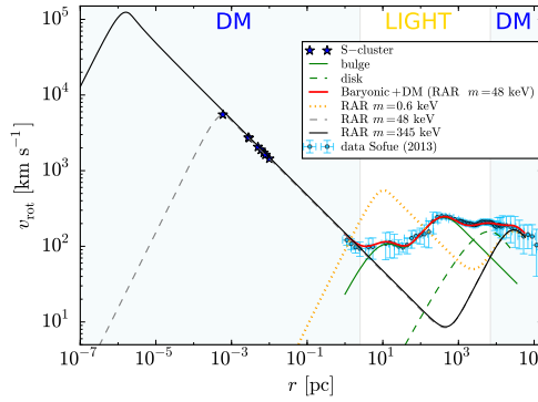
Figure 3.4: (Color online) Theoretical RAR rotation curves from 10^{-7} pc all the way to 10^5 pc, for three representative fermion masses in the mc^2 \sim \text{keV} region: 0.6 keV (dotted yellow curve), 48 keV (long-dashed gray curve) and 345 keV (solid black curve). These RAR solutions are in agreement with all the Milky Way observables from \sim 10^{-3} pc to \sim 10^5 pc. For the case of mc^2 = 48 keV, we include the total rotation curve (red thick curve) including the total baryonic (bulge + disk) component. The star symbols represent the eight best resolved S-cluster stars (Gillessen et al., 2009). See the text for additional details.
