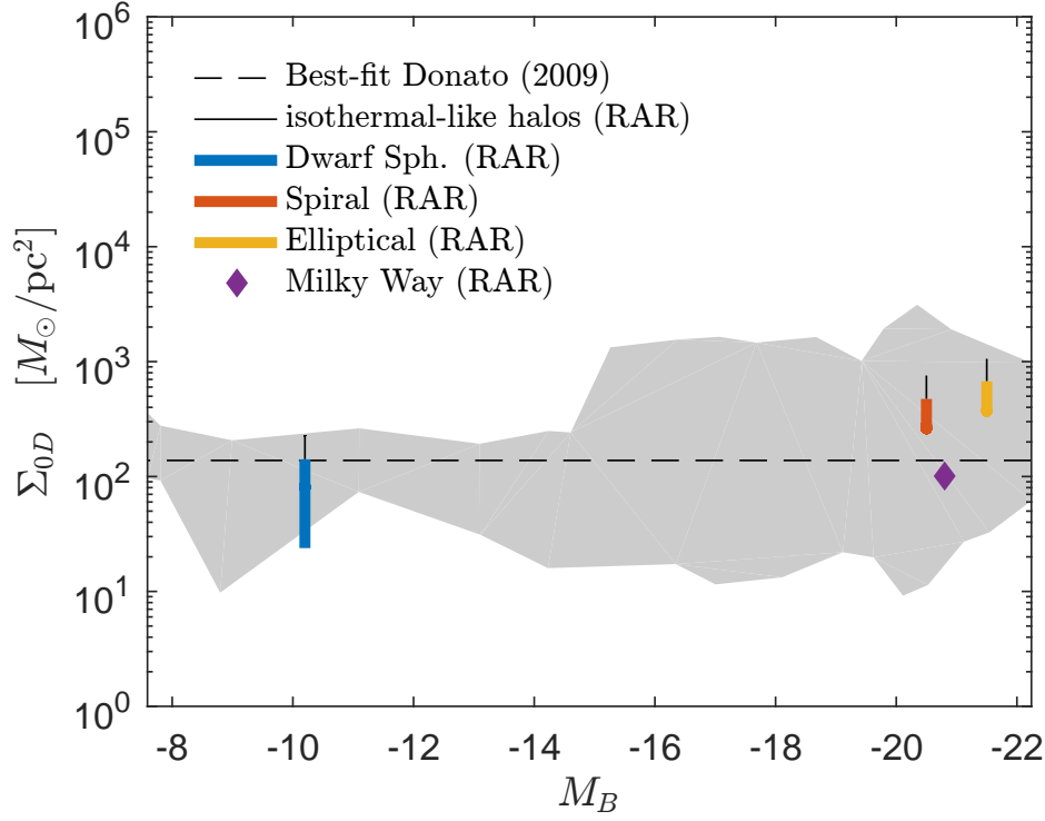
Figure 3.7: (Colour online) The surface DM density as predicted by the RAR model (see vertical colour lines) for each galaxy type in correspondence with the astrophysical RAR family of solutions (i.e. blue-shaded region) given in 3.5. The dashed horizontal line represents the Universal relation as found by Donato et al. (2009) from the best fit of the data. The dark-grey region indicates the delimited area by the 3 - \sigma error bars of all the data points used in Donato et al. (2009). This result shows the ability of the three parametric (\theta_0, \beta_0, W_0) RAR solutions, for mc^2 = 48 \text{ keV} , to be in agreement with the DM surface density observations.
