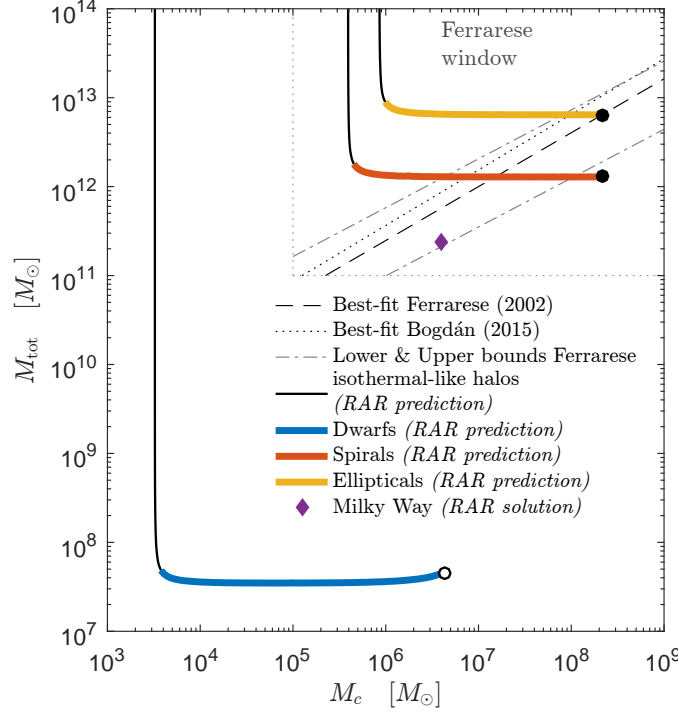
Figure 3.6: (Colour online) The different predicted lines read for each galaxy type in correspondence with the astrophysical RAR family of profiles given in 3.5, showing the ability of the three parametric ( mc^2 = 48 \text{ keV}, \theta_0, \beta_0, W_0 ) RAR solutions to be in agreement with the different M_{\text{BH}} - M_{\text{tot}} relations considered in the literature (see text), and explicated in this picture box. While the red and yellow RAR prediction lines, together to the Milky Way solution (i.e. spiral and elliptical galaxies) lay within the ‘observable Ferrarese window’, the blue RAR prediction for dwarfs, is located at the lower end of the M_c - M_{\text{tot}} plane, where data do not support. The filled-black dots correspond to the critical core masses M_c^{\text{cr}} , and the empty-black dot indicates the limiting maximum core mass for dwarfs M_c^{\text{max}} . The black-continuous lines correspond to RAR solutions having the minimum core mass (or minimum \rho_0 ) which in turn implies the larger cutoff parameters (see Appendix in Argüelles et al. (2018b)), thus developing the more extended and more massive halos.
