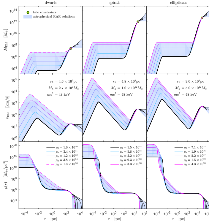
Figure 3.5: (Colour online) Full window of the astrophysical RAR solutions (blue shaded regions enveloped by the 5 benchmark solutions inside), including density profiles (bottom), rotation curves (middle) and DM mass distributions (top); and fulfilling with the observationally given DM halo restriction ( r_h, M_h ) for typical dwarf (left), spiral (middle) and elliptical galaxies (right), for the relevant case of mc^2 = 48 keV. The continuous-magenta curves occurring only for spiral and elliptical galaxies, indicates the critical solutions harboring compact critical cores (before collapsing to a BH) of M_c^{cr} = 2.2 \times 10^8 M_\odot , while the dashed-magenta curves for dwarfs are limited (instead) by the astrophysical necessity of a maximum in the halo rotation curve. The bounding black solutions correspond to the ones having the minimum core mass (or minimum \rho_0 ) which in turn implies the larger cutoff parameters (see Appendix in Argüelles et al. (2018b)), thus developing the more extended density tails allowed by the RAR theory, being \rho \propto r^{-2} the limiting isothermal density tail (achieved when W_0 \rightarrow \infty ).
