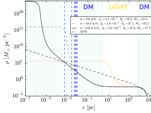
Figure 3.3: (Color online) Theoretical density profiles from 10^{-7} pc all the way to 10^5 pc, for three representative fermion masses in the mc^2 \sim \text{keV} region: 0.6 keV (dotted yellow curve), 48 keV (long-dashed gray curve) and 345 keV (solid black curve). The dashed blue lines indicate the position of the S-cluster stars (Gillessen et al., 2009). We show for the sake of comparison the NFW density profile as obtained in Sofue (2013) (dashed black curve). See the text for additional details.
