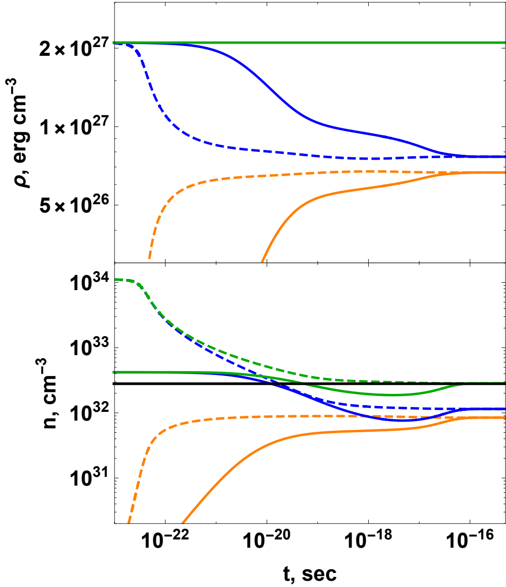
Figure 3.1: Time evolution of energy density, particle number density, chemical potential and temperature of photons (blue), electrons/positrons (orange), all together (green) for relativistic plasma with quantum statistics. Black line represents final equilibrium quantities. Solid and dashed curves correspond to the cases n_{tot}^{in} = 1.5 n_{tot}^{fin} and n_{tot}^{in} = 40 n_{tot}^{fin} , respectively. Final equilibrium temperature is \theta_{fin} = 3 .
