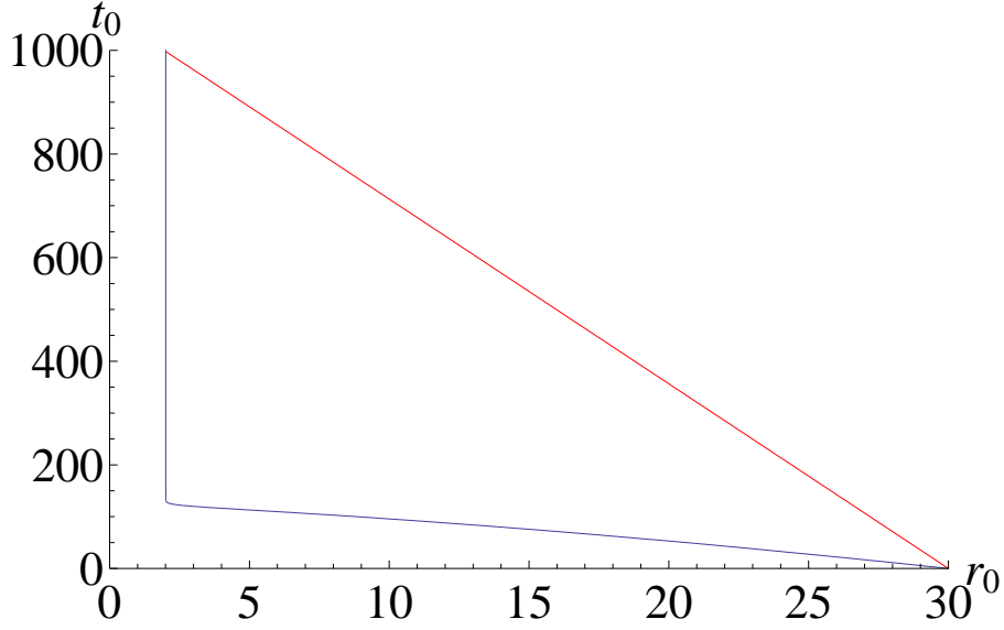
Figure D.2.: In thin shell collapsing process, the time coordinate t_0 is plotted as a function of radial coordinate r_0 of the thin shell. t_0 and r_0 are in unit of GM_0 . The red line is for \xi of Eq. (D.5.2) and the blue for \xi = 0 . The shell is at rest at the radius R_0 = 30 GM_0 and starts to collapse. The thin shell mass M_0 = 20M_\odot .
