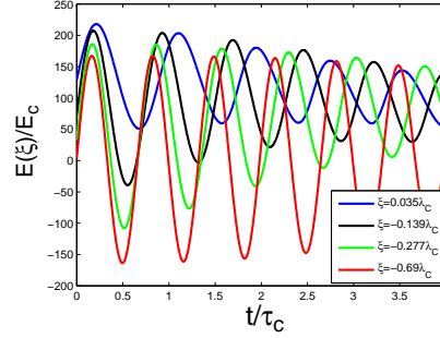
Figure C.2.: Time evolution of electric fields at different radial positions around the boundary layer of the baryon core, M = 10M_\odot , R_c \approx 10^7\text{cm} and v_p = 0.2c . The coordinate is \xi \equiv r - R_c .
