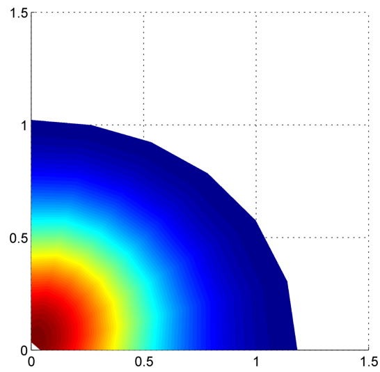
Figure 0.10: 2D density profile of a rotating polytropic star with \gamma = 5/3 in dimensionless variables.
