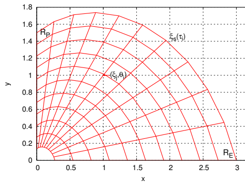
Figure 0.7: Numerical grid used in simulations.
