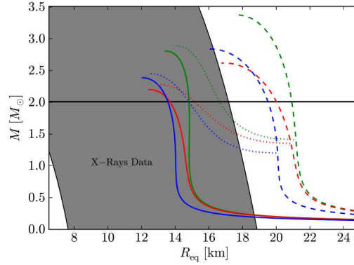
Figure 0.13: Mass versus equatorial radius relation using different equation of state. In addition up-to-date observational constraints are inserted in the figure.
