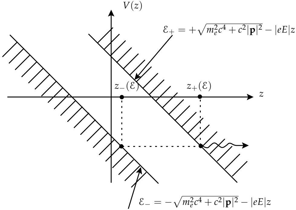
Figure 3.4: Energy-spectra \mathcal{E}_{\pm} with an external electric field \mathbf{E} along \hat{\mathbf{z}} -direction (for -\ell < z < \ell and \ell \gg 1 ). Crossing energy-levels appear, indicated by a dashed line between two continuum energy-spectra \mathcal{E}_- and \mathcal{E}_+ . The turning points z_{\pm}(\mathcal{E}) for the crossing energy-levels \mathcal{E} of Eq. (3.5.5) are marked. This implies that virtual electrons at these crossing energy-levels in the negative energy-spectrum can quantum-mechanically tunnel toward infinity [ z \gg z_+(\mathcal{E}) ] as real electrons; empty states left over in the negative energy-spectrum represent real positrons. This is how quantum tunneling produces pairs of electrons and positrons.
