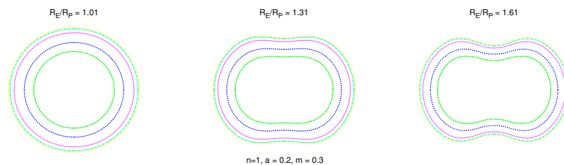
Figure 0.8: Isopicnics for n = 1 with \alpha = 0.2 and \delta^2 = 0.3 for increasing values of the ratio of equatorial and polar radii.
