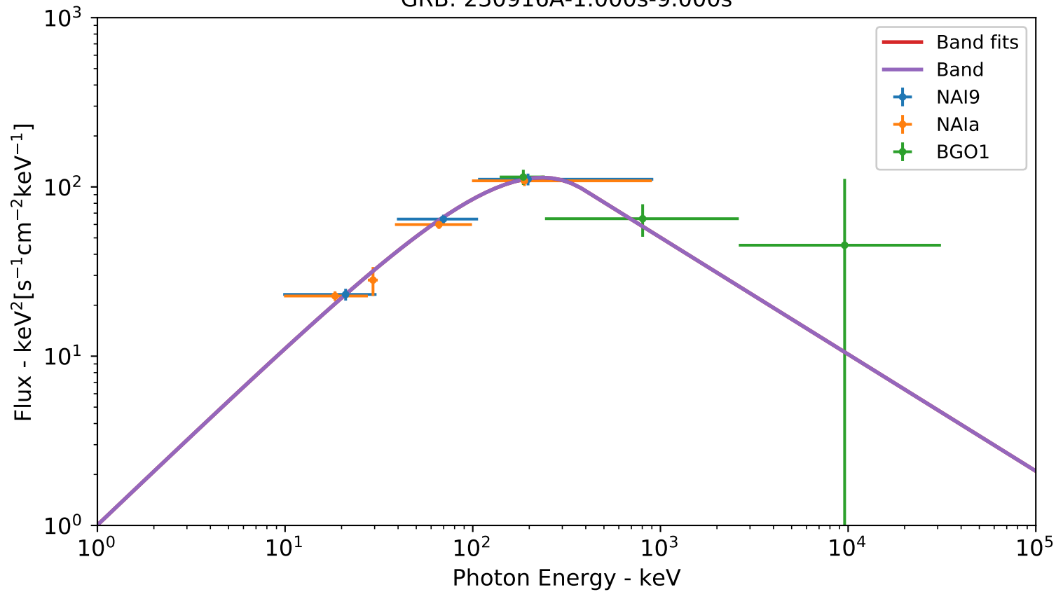
GRB: 230916A-1.000s-9.000s
