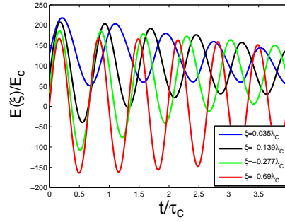
Figure B.2.: Time evolution of electric fields at different radial positions for v_p = 0.1c .
